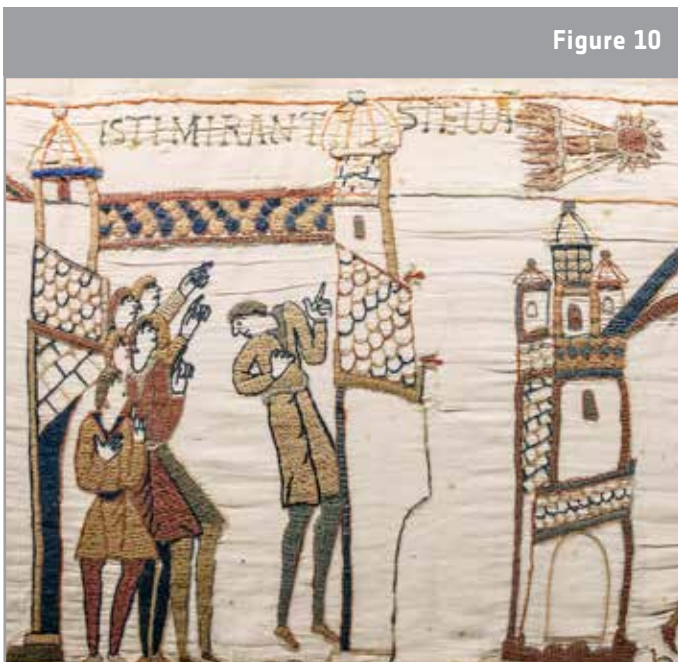
↑ Comet 1P/Halley depicted on the Bayeux tapestry.
