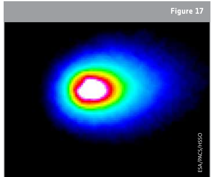
↑ Comet 103P/Hartley as seen by the PACS instrument on the Herschel infrared space observatory.
