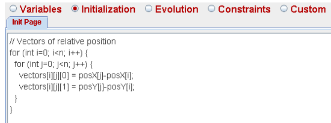
Figure 2.8. Sample initialization code.
