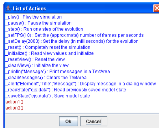
Figure 3.12. List of model methods for an action.
