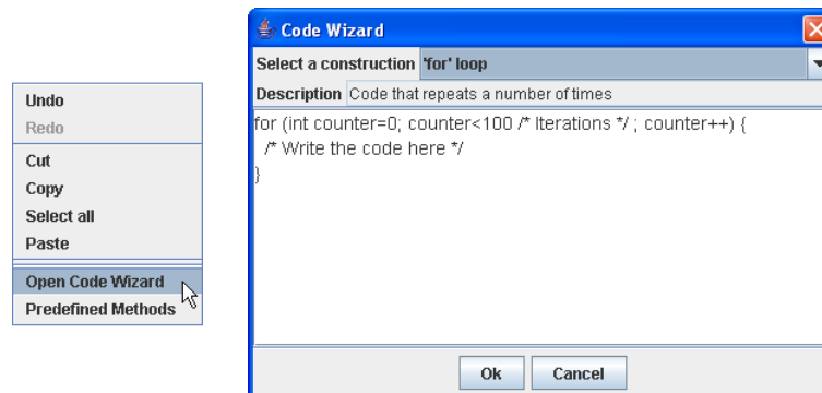
Figure 2.9. Popup menu (left) and code assistant (right).
