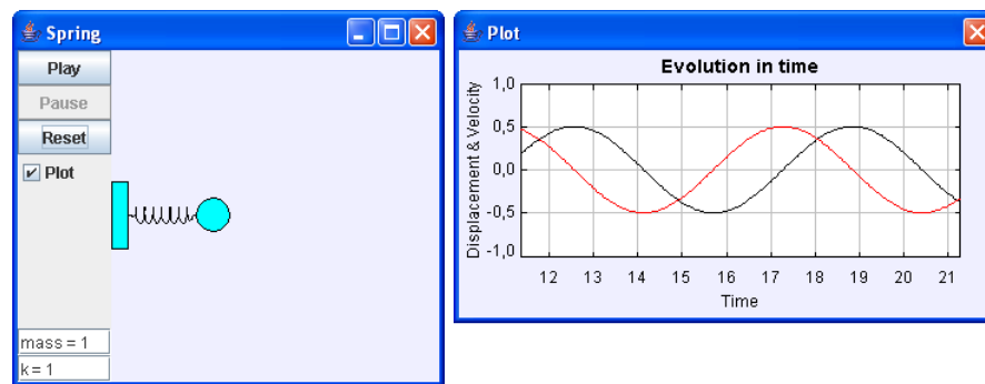
Figure 1.9. The simulation as it runs.
