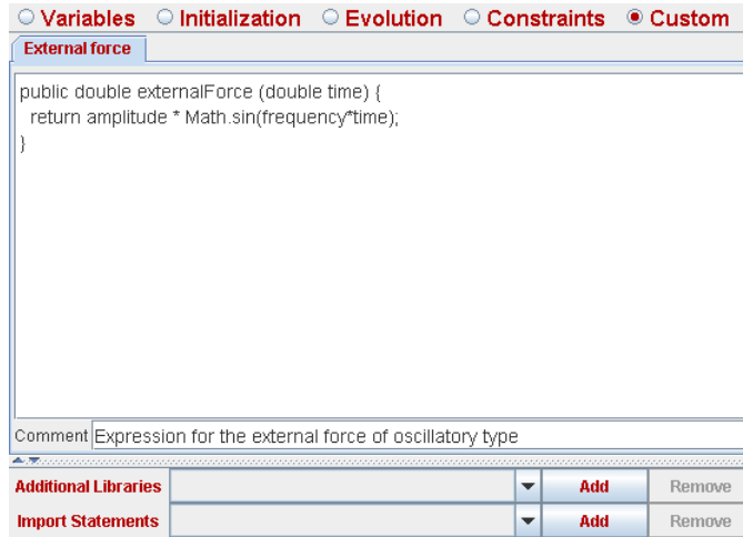
Figure 1.20. Custom method with the expression for the external force.
